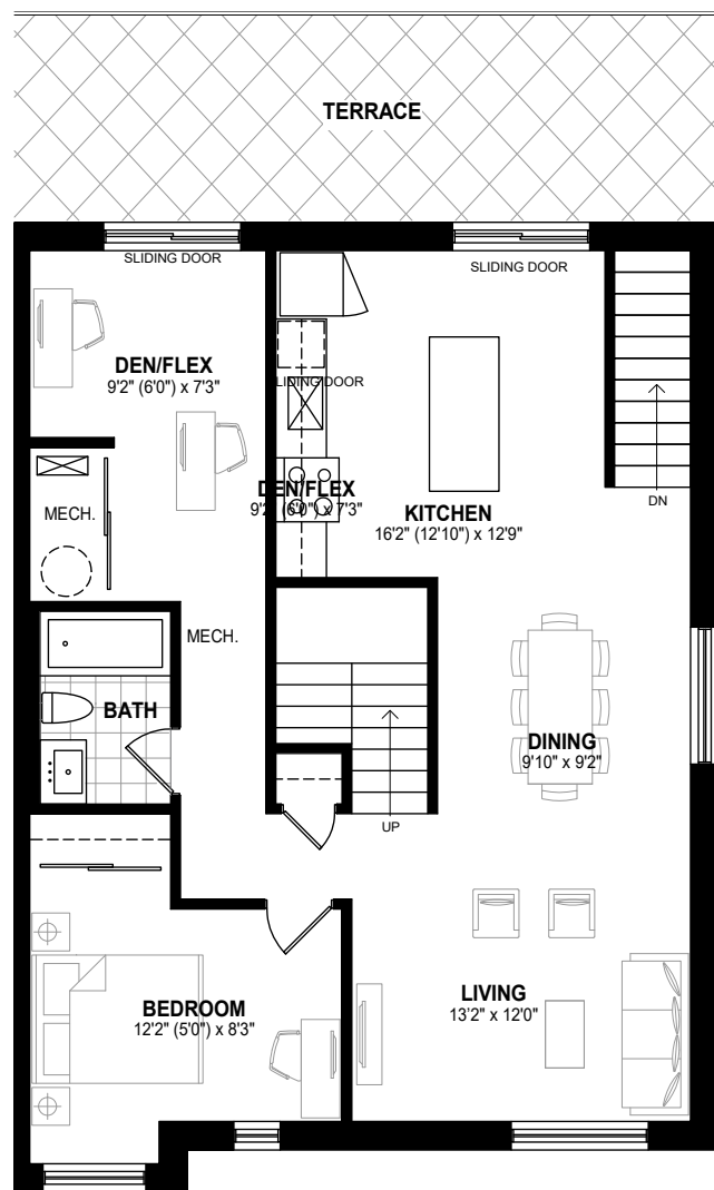
LEVEL 2
