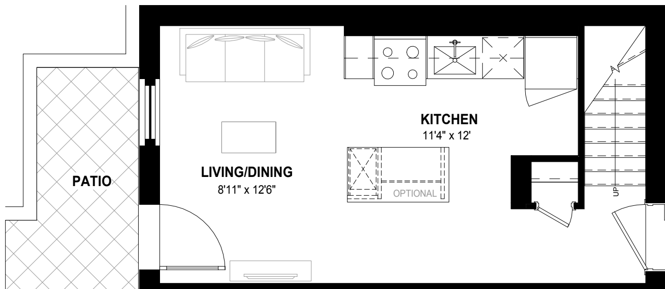
LEVEL 1
