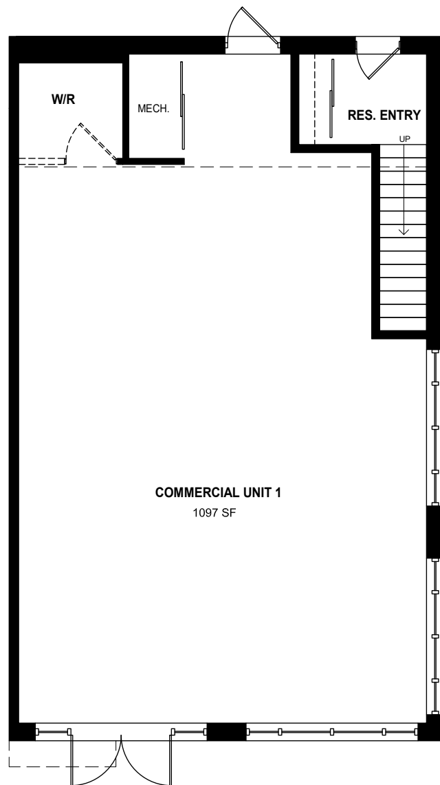
LEVEL 1
