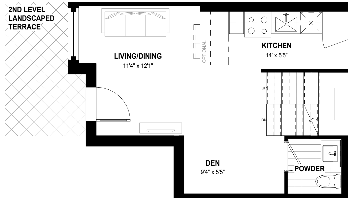
LEVEL 2
