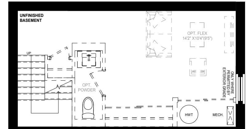
BASEMENT LEVEL
