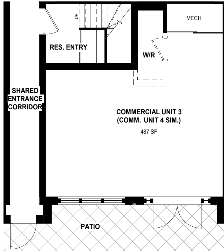
LEVEL 1
